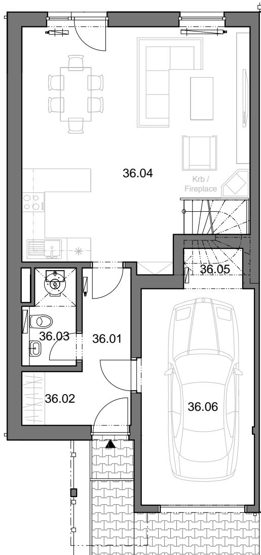
PŮDORYS 1.NP / LAYOUT 1st AGF
