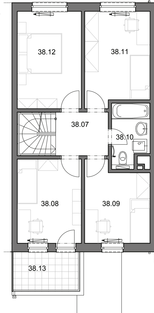
PŮDORYS 2.NP / LAYOUT 2nd AGF
